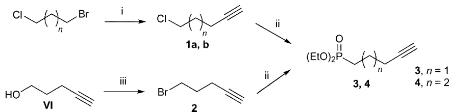
Scheme 3. Synthesis of alkynyl phosphonates. i) \text{HC}\equiv\text{CNa} , liquid \text{NH}_3 , -40^\circ\text{C} , 3 h, 78% ( n = 1 ), 57% ( n = 2 ). ii) \text{P}(\text{OEt})_3 , reflux, 3 d, 34% ( n = 1 ) 3 , 68% ( n = 2 ) 4 . iii) \text{PBr}_3 (0.33 equiv.), pyridine (cat.), diethyl ether, reflux, 2 h, 88%.
